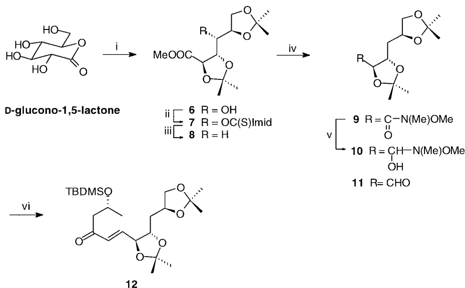
Scheme 3. Reagents: (i) DMP, Acetone, PTSA; (ii) (\text{Imid})_2\text{CS} , 2 equiv, pyridine/ \text{CH}_2\text{Cl}_2 , rt, 18 h; (iii) \text{Bu}_3\text{SnH} , 1.2 equiv, AIBN, degassed toluene, 6 h, 60–65%; (iv) \text{MeNH(OMe)·HCl} 1.6 equiv THF then i -PrMgCl, 3.2 equiv, -20^\circ\text{C} ; (v) \text{LiAlH}_4 , 1.2 equiv THF, 0^\circ\text{C} , 89%; (vi) 5 , 1.5 equiv, \text{Et}_2\text{O} , \text{LiOH·H}_2\text{O} , 2.6 equiv then 10 , \text{Et}_2\text{O} , 82.
