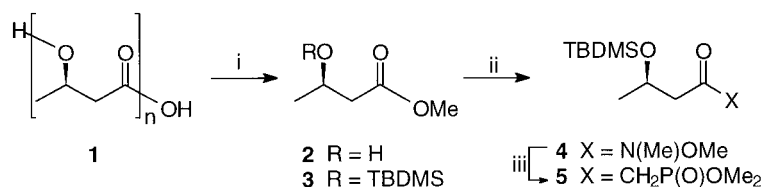
Scheme 2. Reagents: (i) \text{H}_2\text{SO}_4 , 1,2-dichloroethane:MeOH, reflux, 72 h; (ii) TBDMSCl, \text{CH}_2\text{Cl}_2 , \text{NEt}_3 , DMAP; (iii) \text{LiCH}_2\text{P(O)OMe}_2 , THF, -100^\circ\text{C} .
