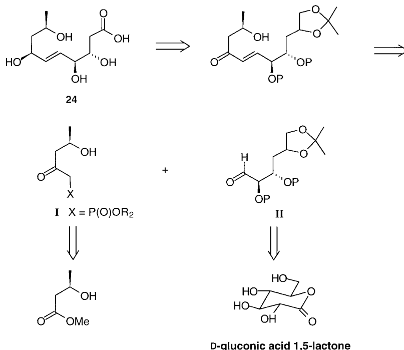
Scheme 1. Retrosynthetic analysis of tuckolide-seco-acid 24 .
