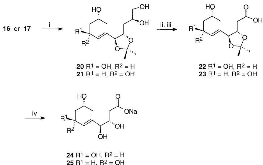
Scheme 5. Reagents: (i) \text{AcOH}:\text{H}_2\text{O}:\text{THF} , 9:1:5, 55 °C, 80%; (ii) \text{NaIO}_4 , 1.5 equiv, \text{MeOH}:\text{H}_2\text{O} ; 2-methyl-2-butene, t BuOH then \text{NaClO}_2 , 6 equiv, \text{NaH}_2\text{PO}_4 , 4.5 equiv in \text{H}_2\text{O} ; (iv) \text{AcOH}:\text{H}_2\text{O}:\text{THF} , 1:1:2, 60 °C, 20 h then \text{NaOH} .
