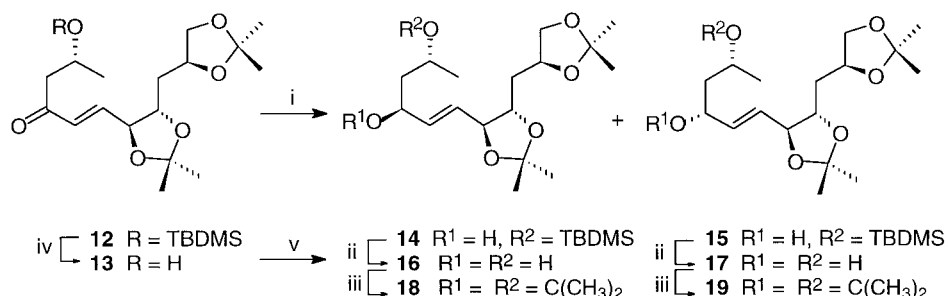
Scheme 4. Reagents: (i) \text{NaBH}_4 , \text{CeCl}_3 , \text{MeOH} , 90%; (ii) TBAF, 1.1 equiv, THF; (iii) DMP, Acetone, PTSA cat., 95% 2 steps; (iv) \text{AcOH}:\text{H}_2\text{O}:\text{THF} , 3:7:20, 4 days, rt; (v) \text{Me}_4\text{NBH}(\text{OAc})_3 , 5 equiv, \text{CH}_3\text{CN}:\text{AcOH} , 1:1.
